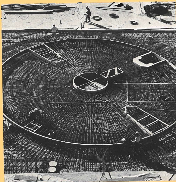
January 1975: Ready for pouring the dome room floor with its radial pattern of reinforcing steel.
