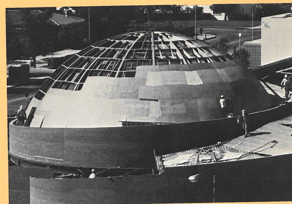
May 1975: A double plywood skin is applied to the dome.
